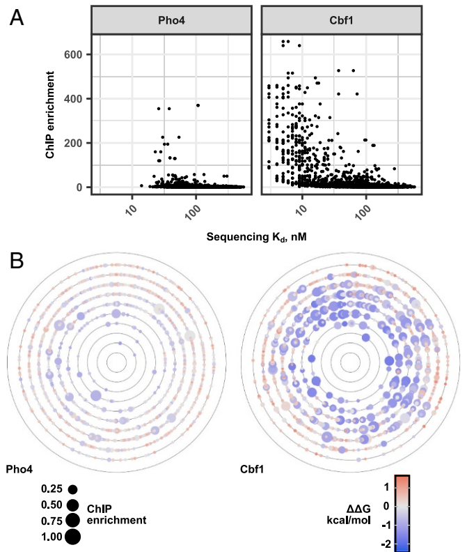
Fig. 5. Pho4 and Cbf1 binding energies and in vivo activity. (A) Pho4 and Cbf1 affinities ( K_d , in nM) compared with in vivo ChIP-seq enrichment (63). (B) Functional-energetic landscapes of ChIP enrichment at dynamically regulated loci, relative to the measured highest affinity sequence in Hamming distance space.
