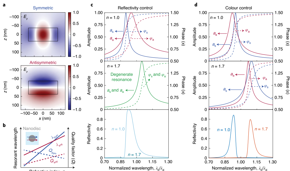
Fig. 2 | Mechanism of dynamic reflectivity and colour control in Si metasurfaces. a , Electric-field distributions ( E_y ) of two dominant optical resonances in a Si nanodisk array with symmetric and antisymmetric radiation profiles. b , Illustration of two dominant optical resonances in nanodisks showing different dispersions with the refractive index of the surrounding medium. Inset: the top view of a unit cell of a nanodisk array supporting two dominant optical resonances. c , Analysis for dynamic reflectivity control by Si metasurfaces. The top and middle panels show the amplitude ( a , solid lines) and phase ( \varphi , dashed lines) of the scattered plane waves from the symmetric (blue) and antisymmetric (red) modes as a function of the incident wavelength when the Si metasurface is embedded in different dielectric environments ( n=1.0 (1.7) for the top (middle) panel). The bottom panel shows the calculated reflection spectra of the metasurface for dynamic reflectivity control. d , Similar analysis to c but for dynamic colour control. The designed wavelength \lambda_d is set as 550 nm.
