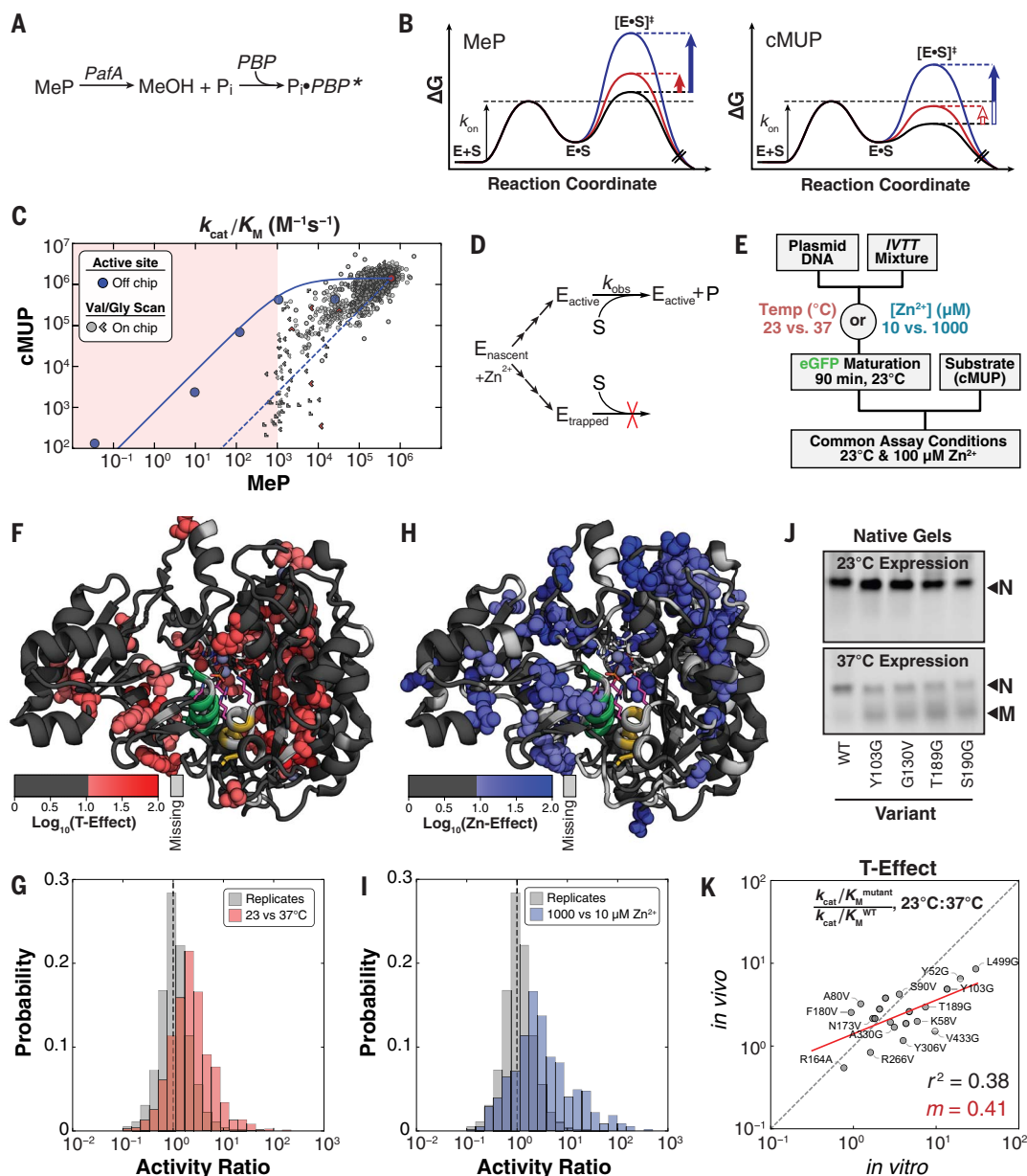
Fig. 3. Substrates with different intrinsic reactivity reveal kinetic folding traps. (A) Schematic illustrating real-time detection of P_i produced by MeP hydrolysis on-chip using a fluorophore-conjugated PBP (18). (B) Reaction coordinate diagrams schematically illustrating substrates with either chemistry (MeP) or binding (cMUP) as the rate-limiting step. Solid arrows indicate observable mutational effects on the chemical step, and open arrows indicate effects that are not observable. (C) Measured k_{cat}/K_M for MeP versus k_{cat}/K_M for cMUP for active-site mutants off-chip (blue points) and for valine and glycine mutants. Limits in one or both directions are indicated with chevrons pointing in the direction or quadrant of the limit. The red shaded region denotes lower limit of detection for MeP, the solid blue line indicates predicted relationship between k_{cat}/K_M for cMUP and MeP hydrolysis, and the dashed blue line shows predicted relationship for enzymes with WT activity but a varying fraction of inactive enzyme (supplementary text S2). (D) Scheme showing kinetic partitioning between folded (active) and misfolded (kinetically trapped) enzyme during expression. (E) Pulse-chase experiment to test for expression-dependent misfolding by varying expression conditions while keeping reaction conditions constant. (F) Residues with temperature-dependent activity changes shown
